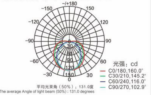
配光曲线图/Light distribution curve
