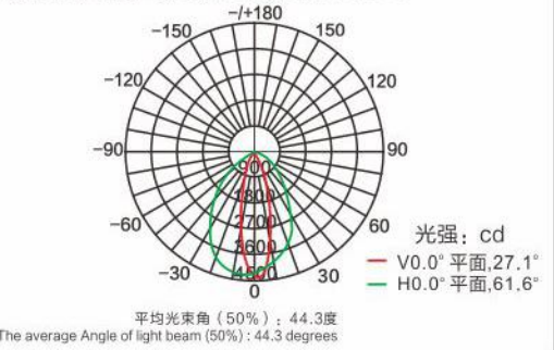
配光曲线图/Light distribution curve
