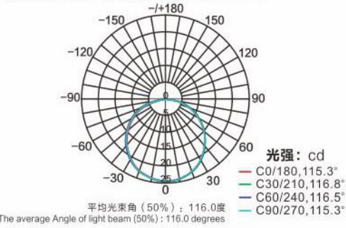
配光曲线图/Light distribution curve
